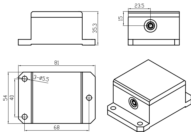
Picture 3 SSL100 with Binder712 connector
