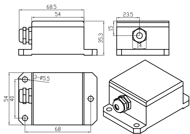
Picture 4 SSL100 with metal pigtail
