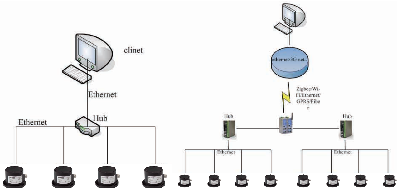
Picture 1 Inclinator measuring system (LAN)
